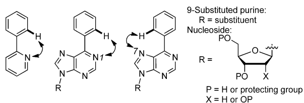
Scheme 1. N-directed C–H bond activation in 2-phenylpyridine, and two plausible modes of N-directed C–H bond activation in C6-aryl purines and nucleosides.
