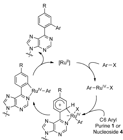
Scheme 3. Possible mechanism for the C–H bond activation/arylation of 6-aryl purine and 6-aryl purine 2'-deoxyribonucleosides.
