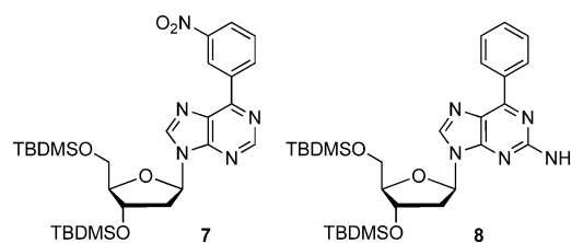
Scheme 2. Nucleoside substrates that did not yield arylation products. TBDMS = tert -butyldimethylsilyl.
