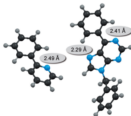
Figure 1. Energy-minimized structures of 2-phenylpyridine (left) and 9-benzyl-6-phenyl-9 H -purine (right).
